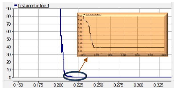
Fig. 6. 1 st agent decision signal ( 2\phi , 30\Omega fault in L1)
