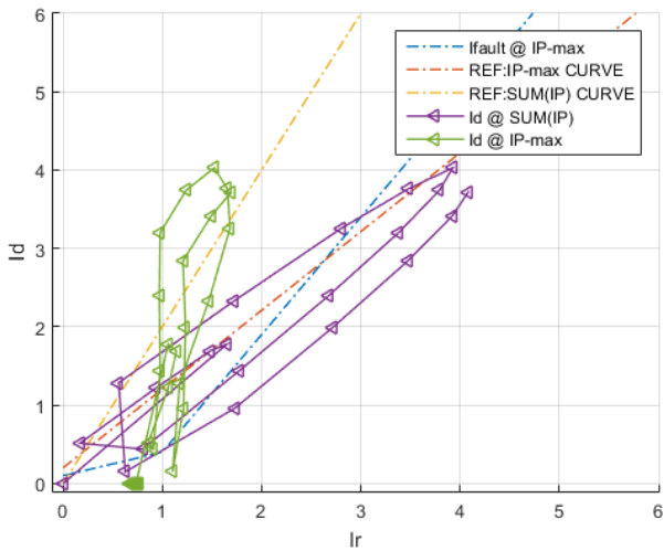
Fig. 8. REF curves for in-zone single-phase fault
