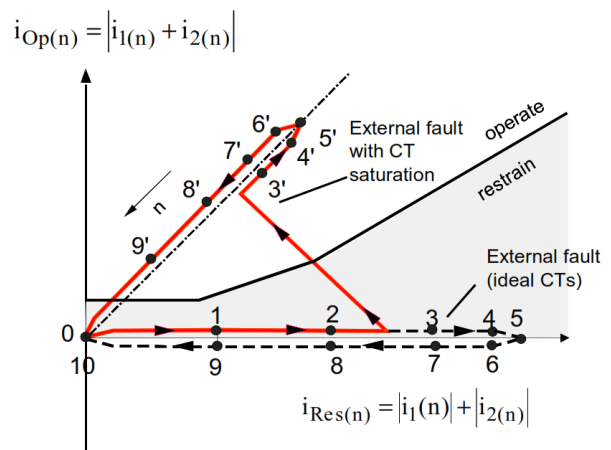
Fig. 6. Movement of operating point in REF curve with/without CT saturation
