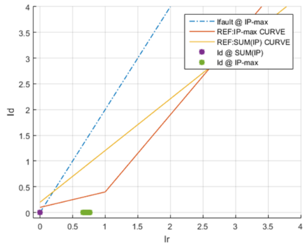
Fig. 7. SUM (IP) and IP-MAX mode's curves
