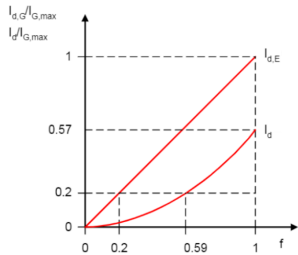
Fig. 2. DIFF and REF fault current for Dyn transformer
