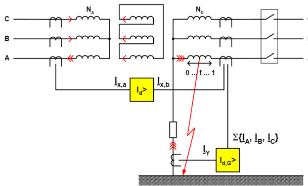
Fig. 1. REF and differential protection scheme
