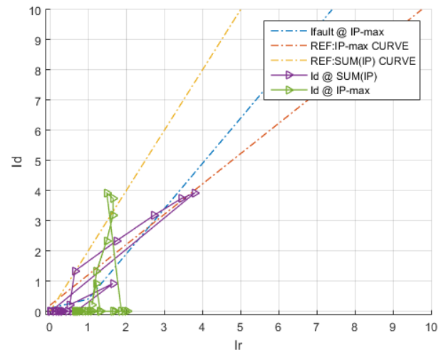
Fig. 9. REF operation curve for an out zone single phase fault with CTs saturation condition
