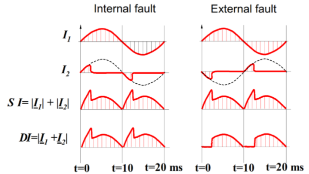
Fig. 5. In/out zone fault current during CT saturation
