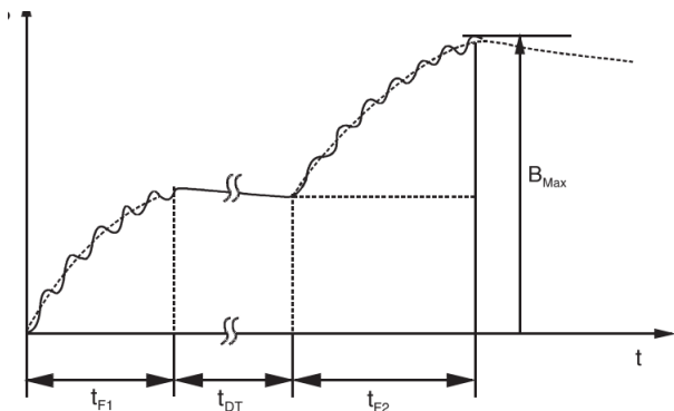
Fig. 4. Effect of reclosing on CT flux remanence
