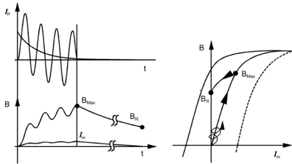
Fig. 3. The remanence flux in the CT core
