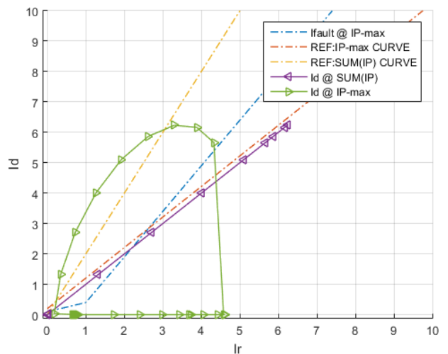
Fig. 10. REF curve for out-zone two/three phase faults with CTs saturation condition
