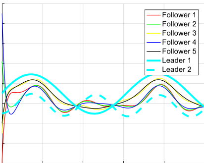
Fig. 13. Formation-containment with dynamic leaders and h_i^F = 0.2 \cos(\pi t + \frac{k_i\pi}{7}) .
