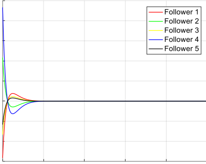
Fig. 10. Containment error with dynamic leaders.
